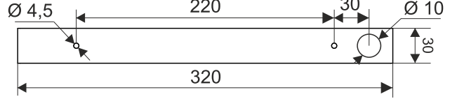
THIN TUBE 68-152 LED hermetic wall:
